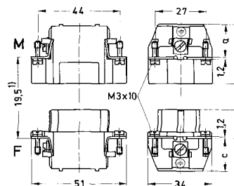
Drawing Dimensions in mm
